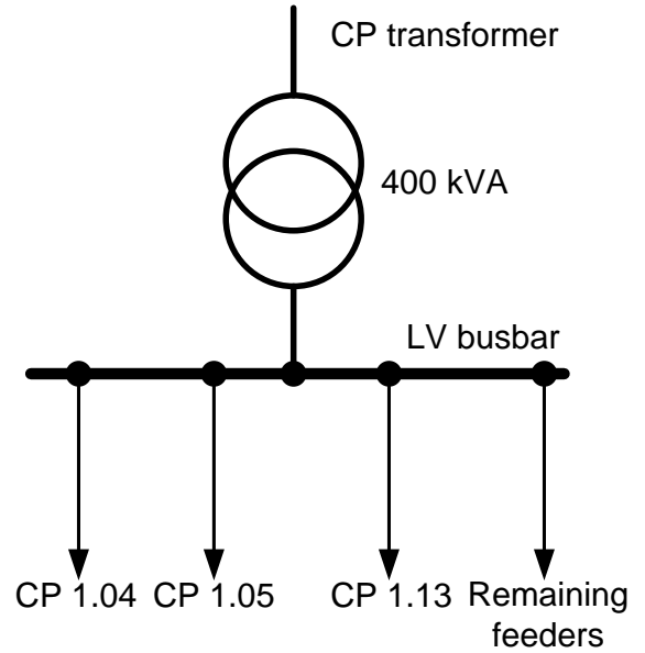
Fig 14: Secondary substation layout including congestion points
